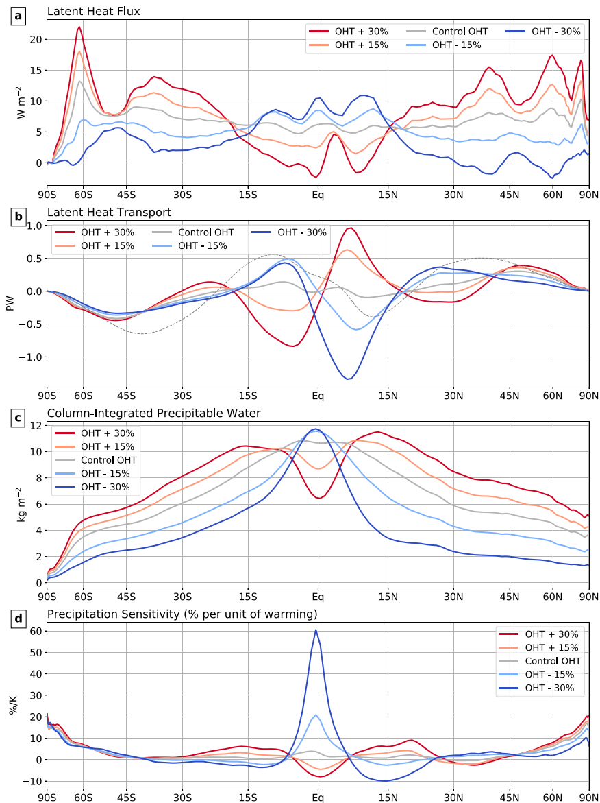
FIG. 12. Zonal mean change in the atmospheric hydrologic cycle in the CESM1-SOM CO_2 -doubling experiments, relative to the preindustrial control: (a) change in the surface latent heat flux ( W m^{-2} ); (b) change in the latent heat transport (in PW; the black dotted line shows the latent heat transport in the preindustrial control, scaled by a factor of 0.1); (c) change in column-integrated precipitable water ( kg m^{-2} ); and (d) the precipitation sensitivity, the percentage change in precipitation relative to the global mean surface temperature change ( \% K^{-1} ).
